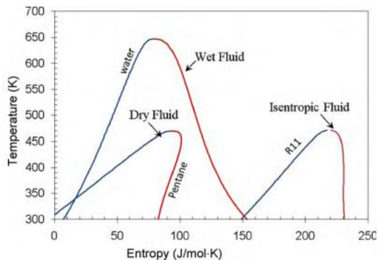
Figure 3. T-s diagram of the three main groups of working fluids (Chen et al., 2010).
