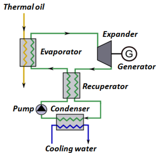
Figure 5. Layout of the ORC.
